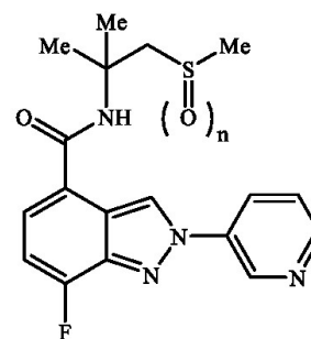
Compound of Formula 2
